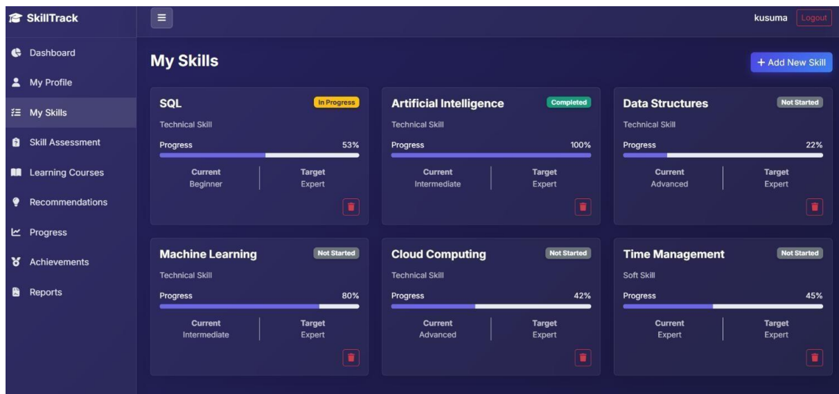
Figure 6 – My Skills
